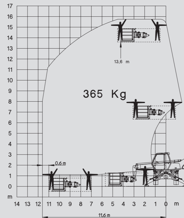
ROTATION ON STABILISERS WITH 365 KG PLATFORM ORH - 2/4 m
