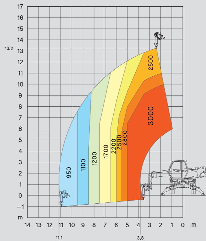
ROTATION ON STABILISERS WITH 3T WINCH
