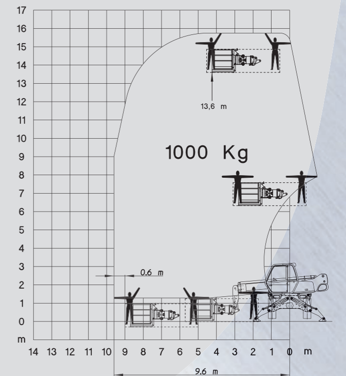
ROTATION ON STABILISERS WITH 1000 KG PLATFORM ORH - 2/4 m
